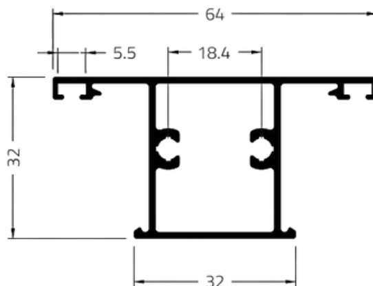
TRAVESSA MAXIM-AR GOLD
