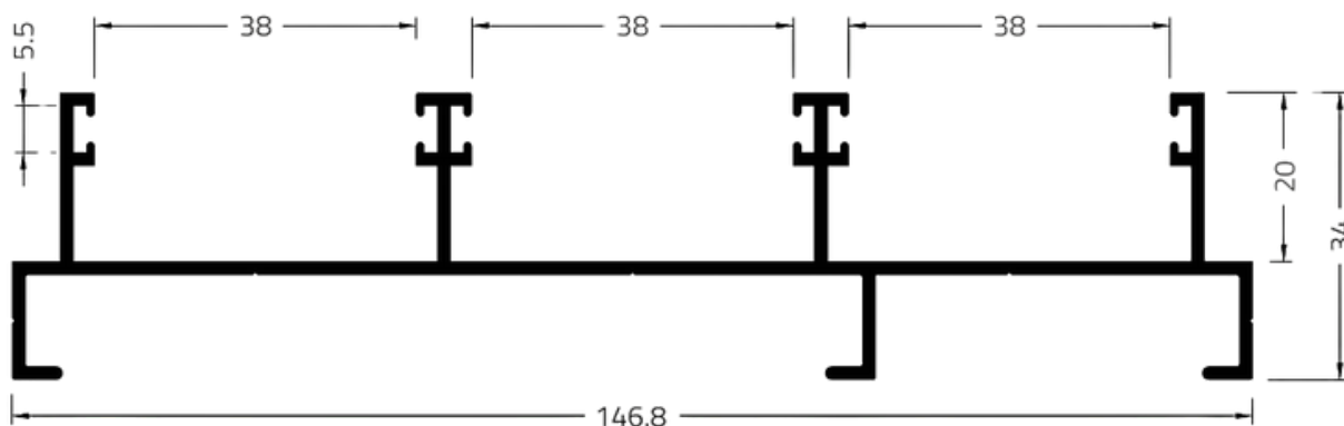
MARCO LATERAL 3 PLANOS GOLD
