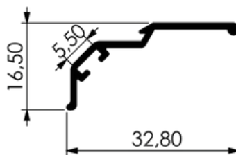
PINGADEIRA MAXIM-AR
