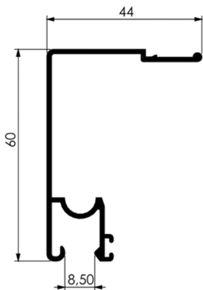
TRILHO SUP V 8MM (LEVE)
