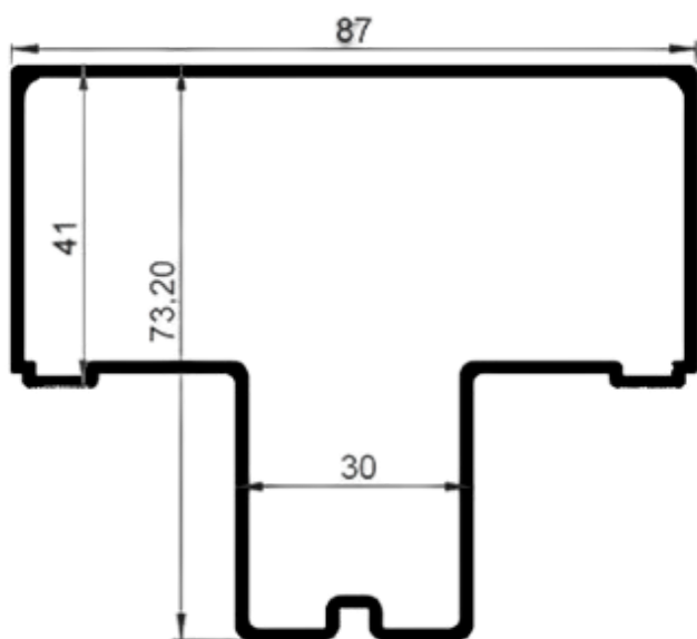
COLUNA CENTRAL FACHADA 41 MM
