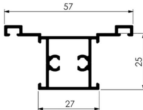
TRAVESSA MAXIM-AR
