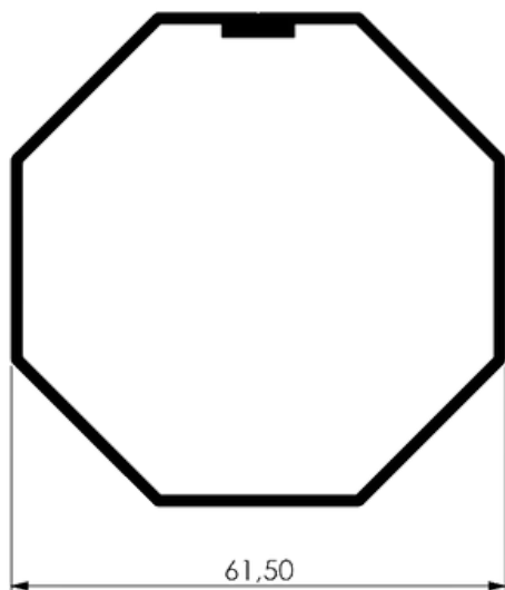
TUBO OCTAGONAL INTEGRADA 60MM
