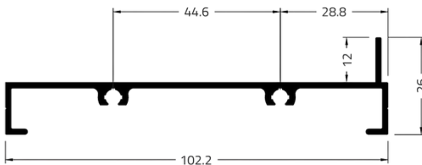
MARCO BANDEIRA GOLD
