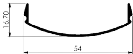
ARREIMATE DE CORRIMÃO (CLICK)
