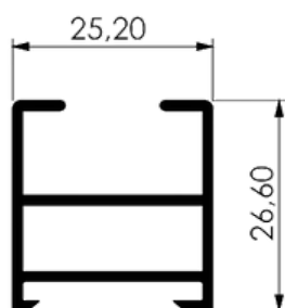
TRAVESSA SUPERIOR
